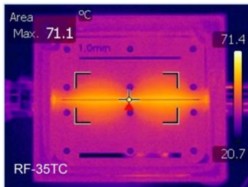
Thermal image of a microstrip transmission line with 0805 capacitor at center (47pF/250V/C0G) assembled on RF-35TC under 200 watts applied power.
